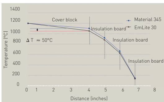
◀ Fig 2. Heat Loss as calculated by Steady-State Heat Flow comparing Em-Lite 30 and Material 345.
